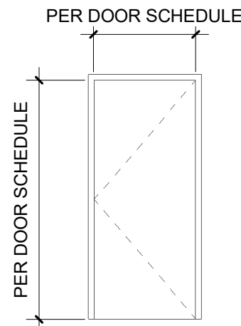
B EXISTING RELOCATED RATED SOLID CORE WD DOOR WITH RATED HM FRAME
